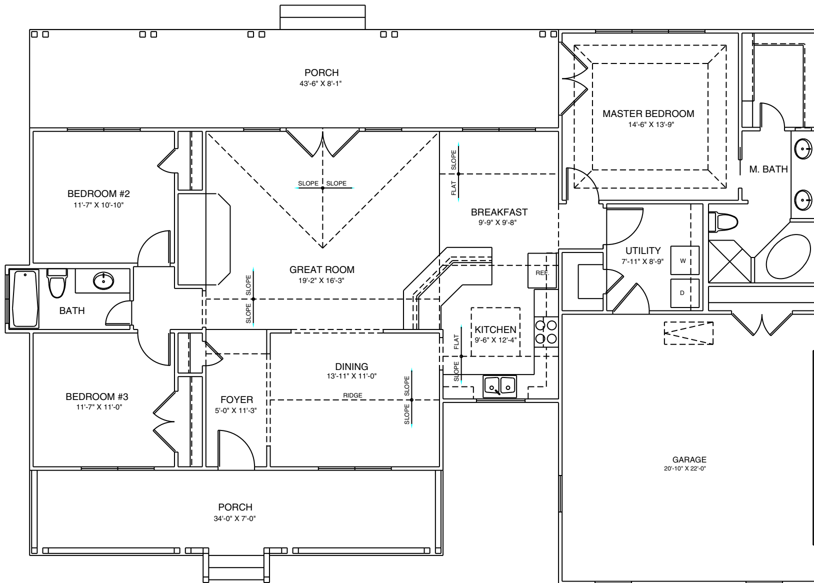
FLOOR PLAN
